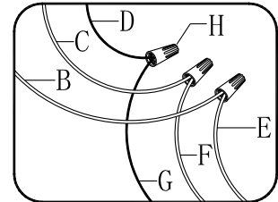
Wire connection
